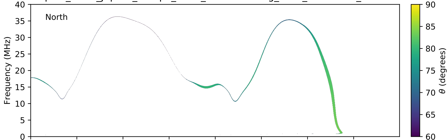
expres_earth_jupiter_europa_isaac_lossc-wid1deg_3kev_20160525_v01.cdf
