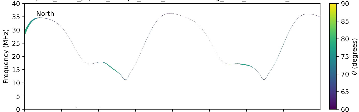
expres_earth_jupiter_europa_isaac_lossc-wid1deg_3kev_20160521_v01.cdf
