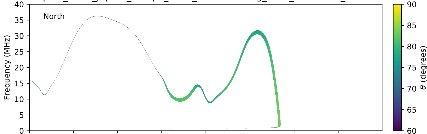
expres_earth_jupiter_europa_isaac_lossc-wid1deg_3kev_20160511_v01.cdf
