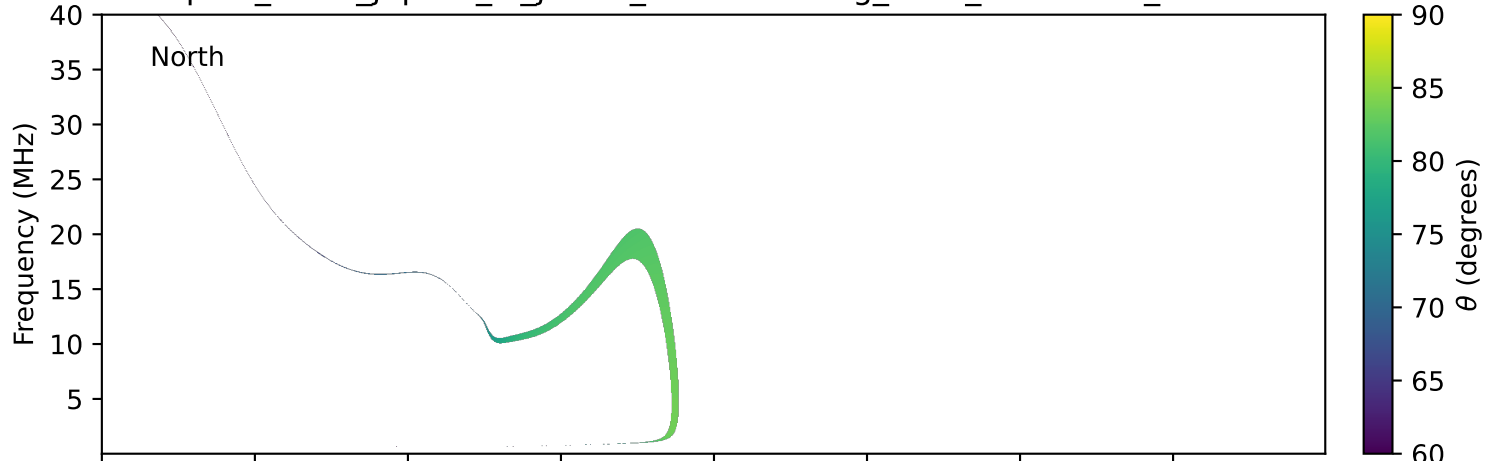
expres_earth_jupiter_io_jrm33_lossc-wid1deg_3kev_20160423_v11.cdf
