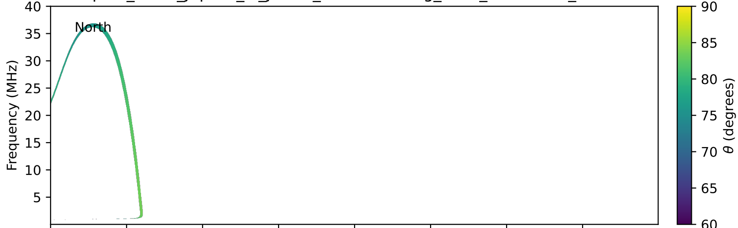
expres_earth_jupiter_io_jrm33_lossc-wid1deg_3kev_20160418_v11.cdf
