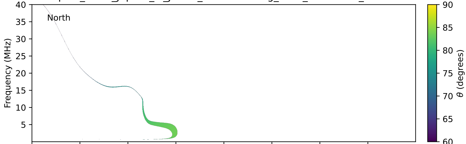
expres_earth_jupiter_io_jrm33_lossc-wid1deg_3kev_20160416_v11.cdf
