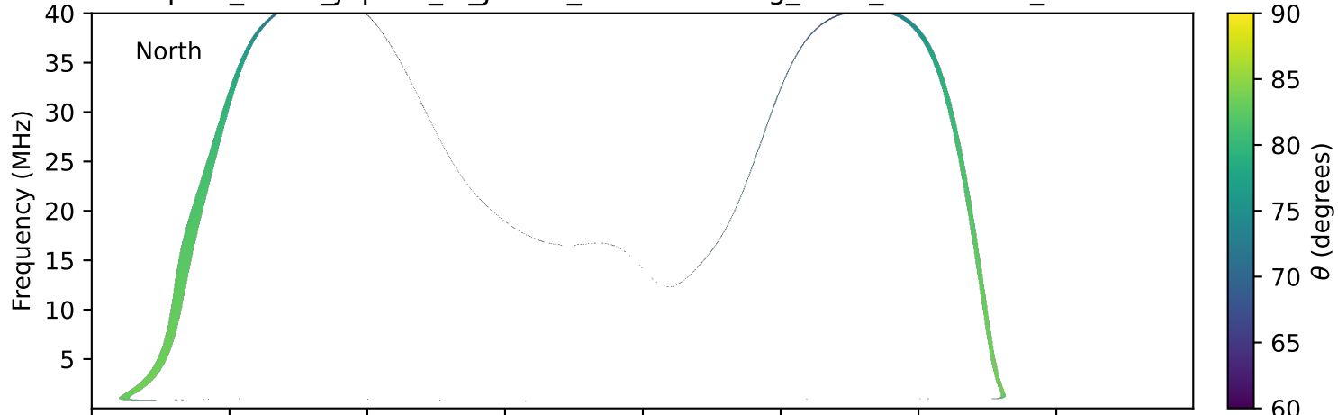
expres_earth_jupiter_io_jrm33_lossc-wid1deg_3kev_20160412_v11.cdf
