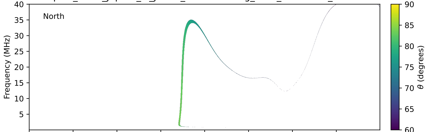
expres_earth_jupiter_io_jrm33_lossc-wid1deg_3kev_20160401_v11.cdf
