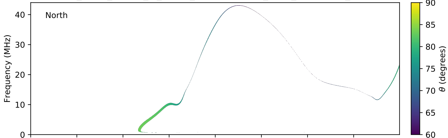
expres_earth_jupiter_io_jrm09_lossc-wid1deg_3kev_20160417_v01.cdf
