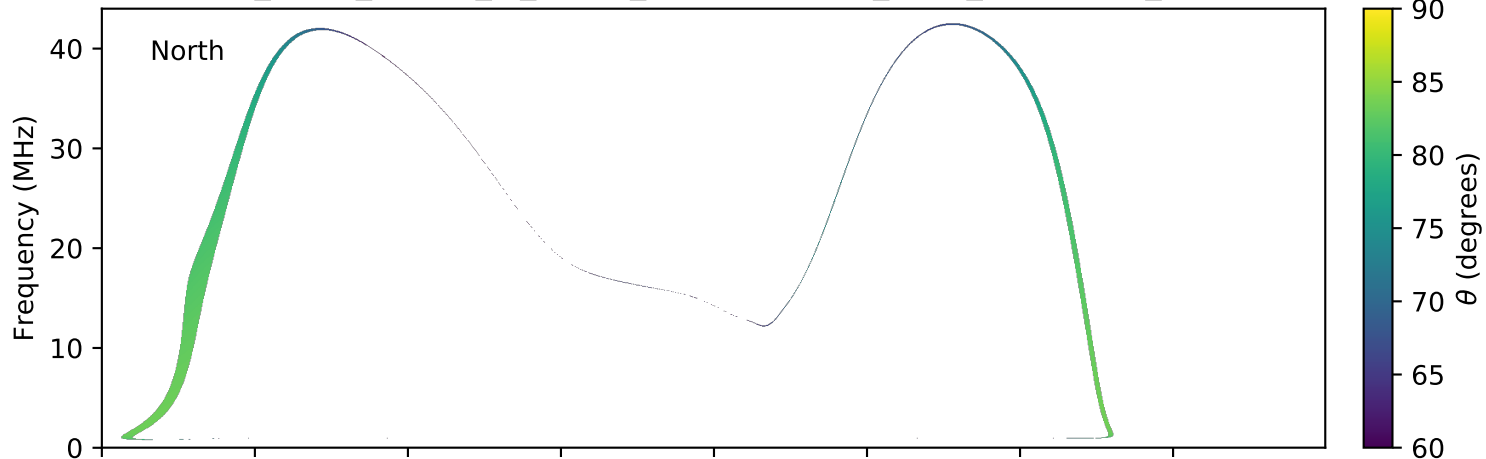
expres_earth_jupiter_io_jrm09_lossc-wid1deg_3kev_20160412_v01.cdf
