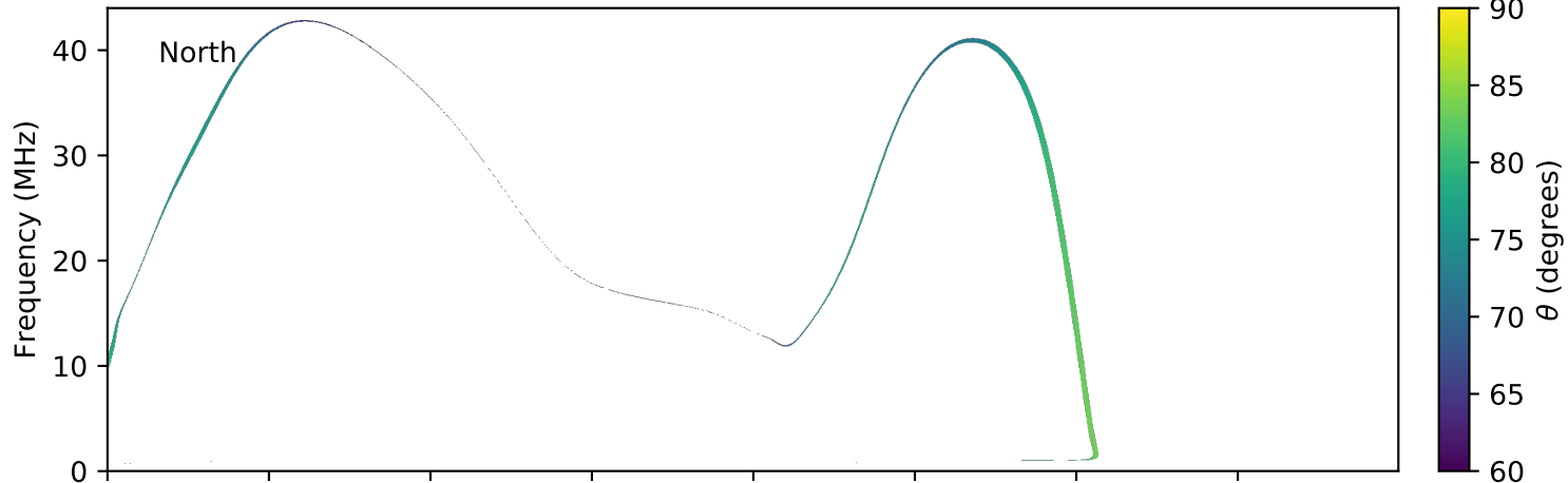
expres_earth_jupiter_io_jrm09_lossc-wid1deg_3kev_20160405_v01.cdf
