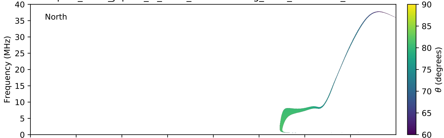
expres_earth_jupiter_io_isaac_lossc-wid1deg_5kev_20160429_v01.cdf
