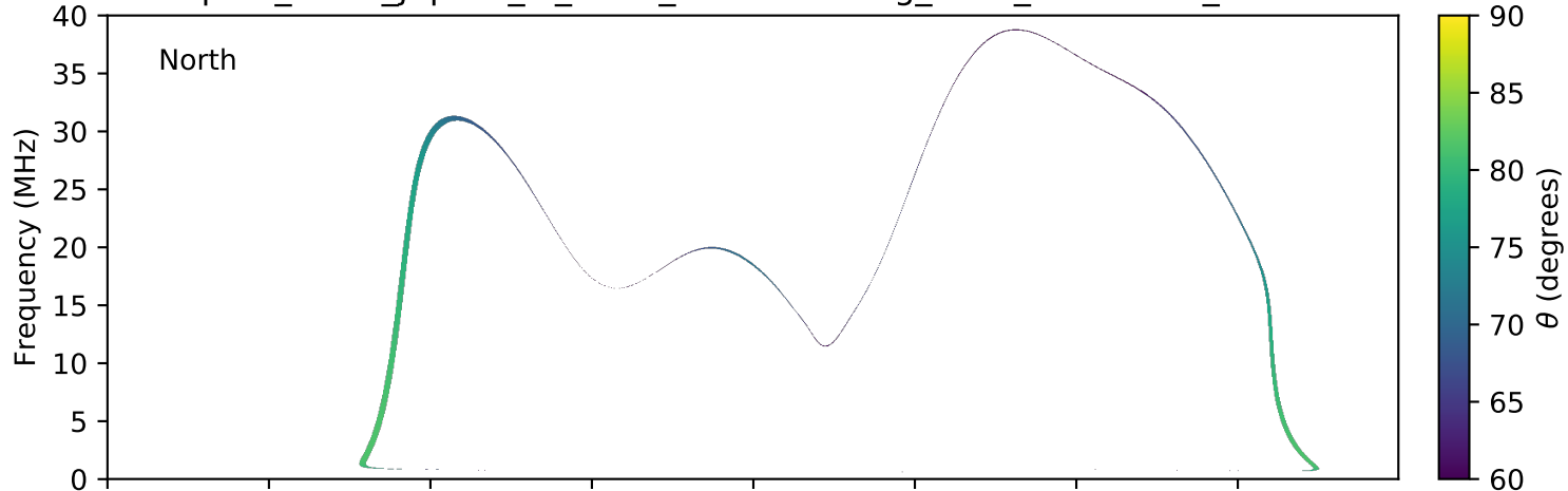
expres_earth_jupiter_io_isaac_lossc-wid1deg_5kev_20160426_v01.cdf
