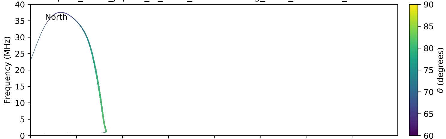
expres_earth_jupiter_io_isaac_lossc-wid1deg_5kev_20160425_v01.cdf
