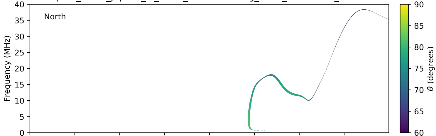
expres_earth_jupiter_io_isaac_lossc-wid1deg_5kev_20160422_v01.cdf
