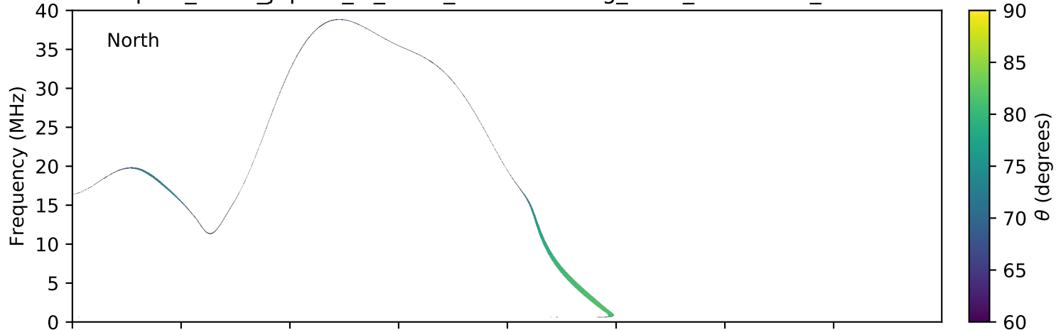
expres_earth_jupiter_io_isaac_lossc-wid1deg_5kev_20160421_v01.cdf
