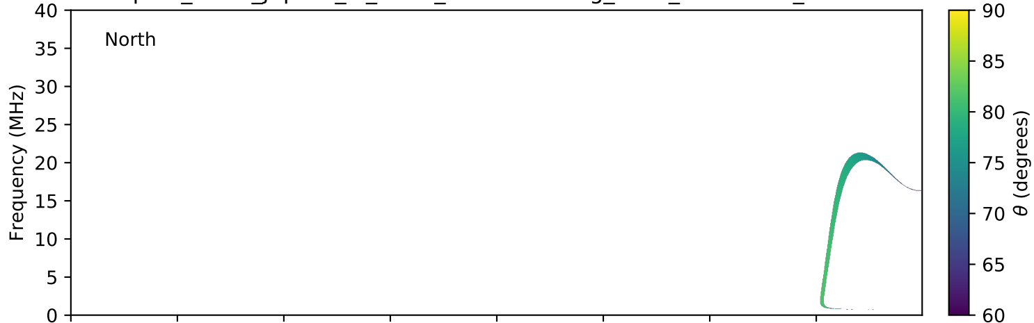
expres_earth_jupiter_io_isaac_lossc-wid1deg_5kev_20160420_v01.cdf
