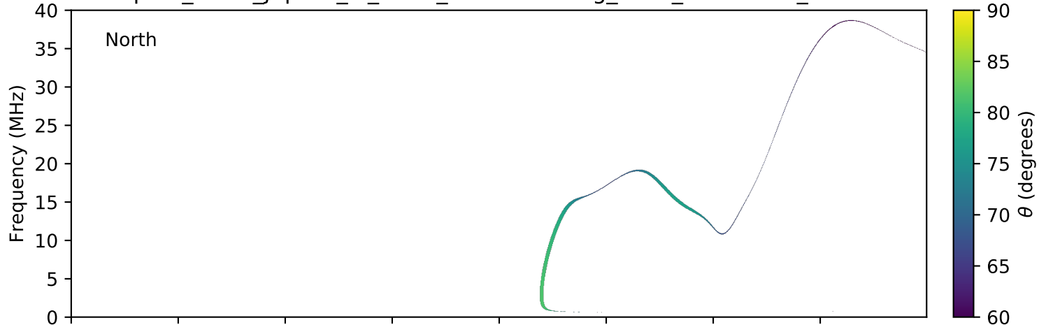
expres_earth_jupiter_io_isaac_lossc-wid1deg_5kev_20160415_v01.cdf
