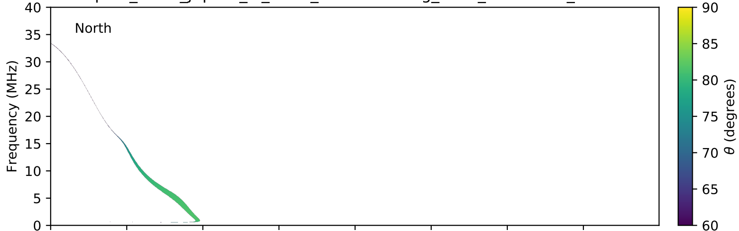
expres_earth_jupiter_io_isaac_lossc-wid1deg_5kev_20160409_v01.cdf
