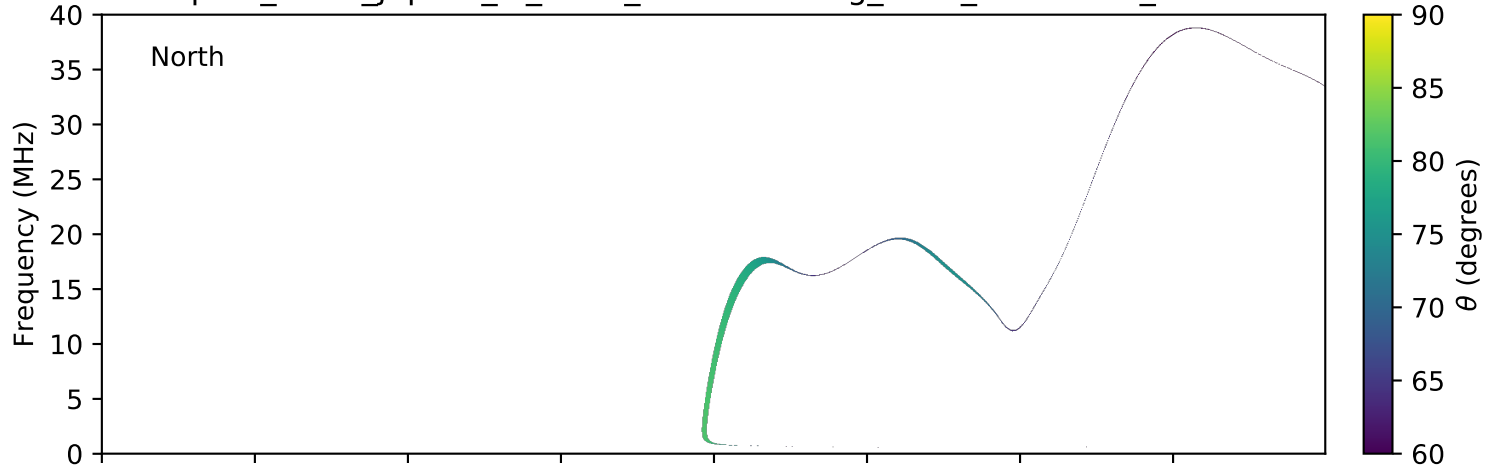
expres_earth_jupiter_io_isaac_lossc-wid1deg_5kev_20160408_v01.cdf
