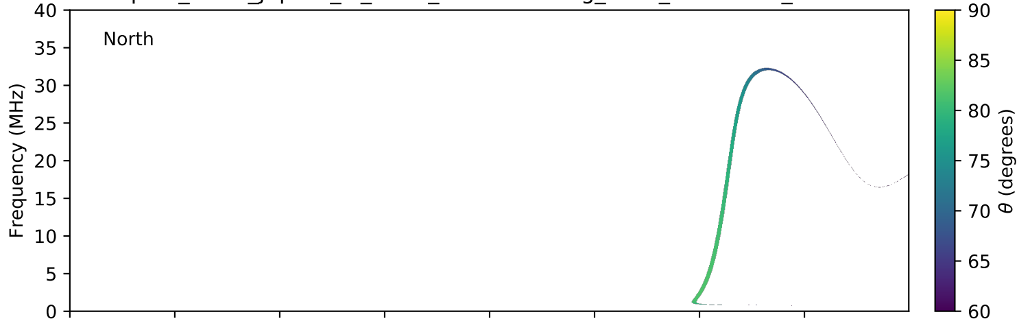
expres_earth_jupiter_io_isaac_lossc-wid1deg_5kev_20160406_v01.cdf
