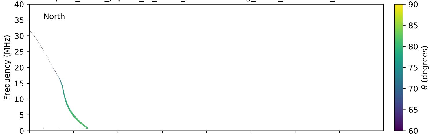
expres_earth_jupiter_io_isaac_lossc-wid1deg_5kev_20160402_v01.cdf
