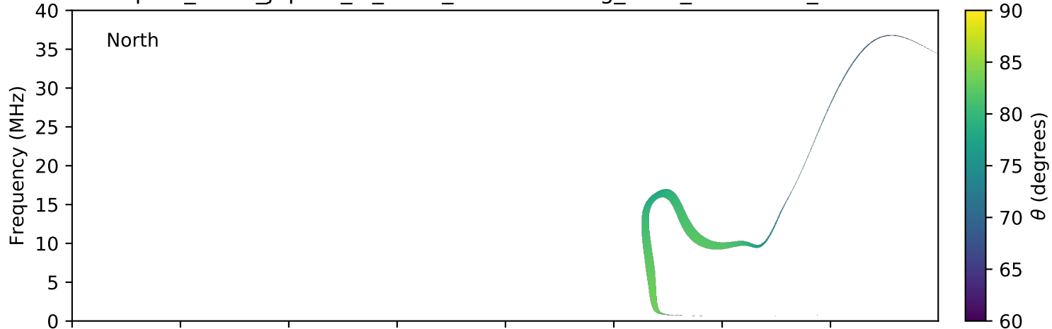
expres_earth_jupiter_io_isaac_lossc-wid1deg_3kev_20160429_v01.cdf
