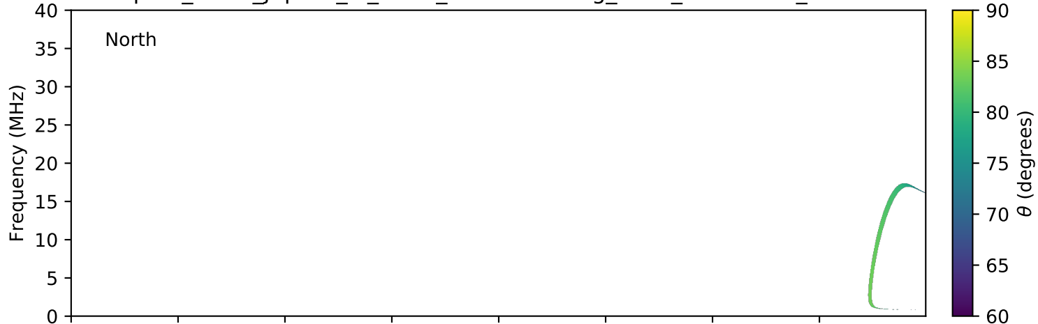
expres_earth_jupiter_io_isaac_lossc-wid1deg_3kev_20160427_v01.cdf
