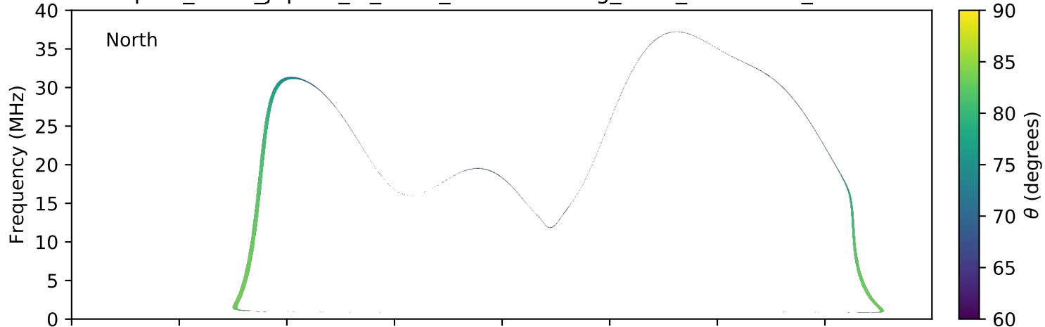
expres_earth_jupiter_io_isaac_lossc-wid1deg_3kev_20160426_v01.cdf
