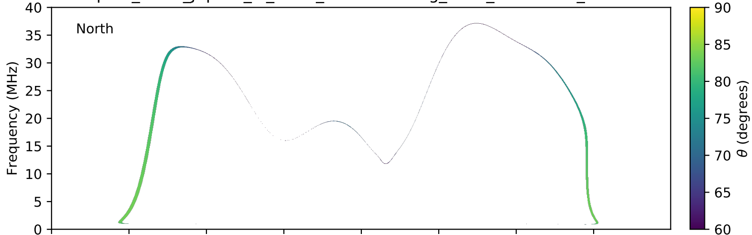
expres_earth_jupiter_io_isaac_lossc-wid1deg_3kev_20160419_v01.cdf
