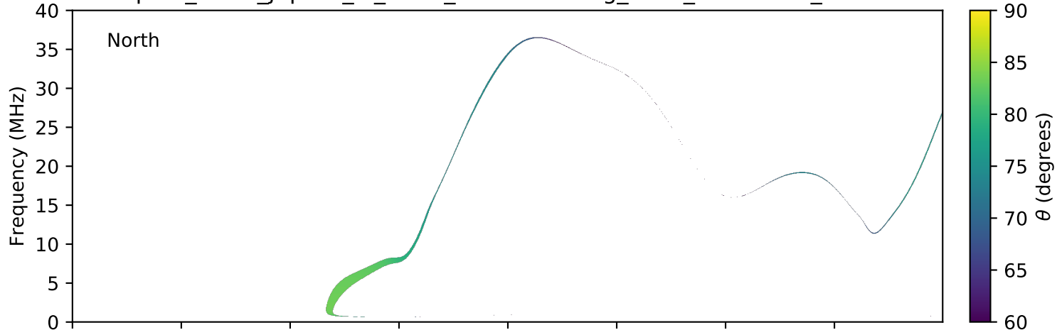
expres_earth_jupiter_io_isaac_lossc-wid1deg_3kev_20160417_v01.cdf
