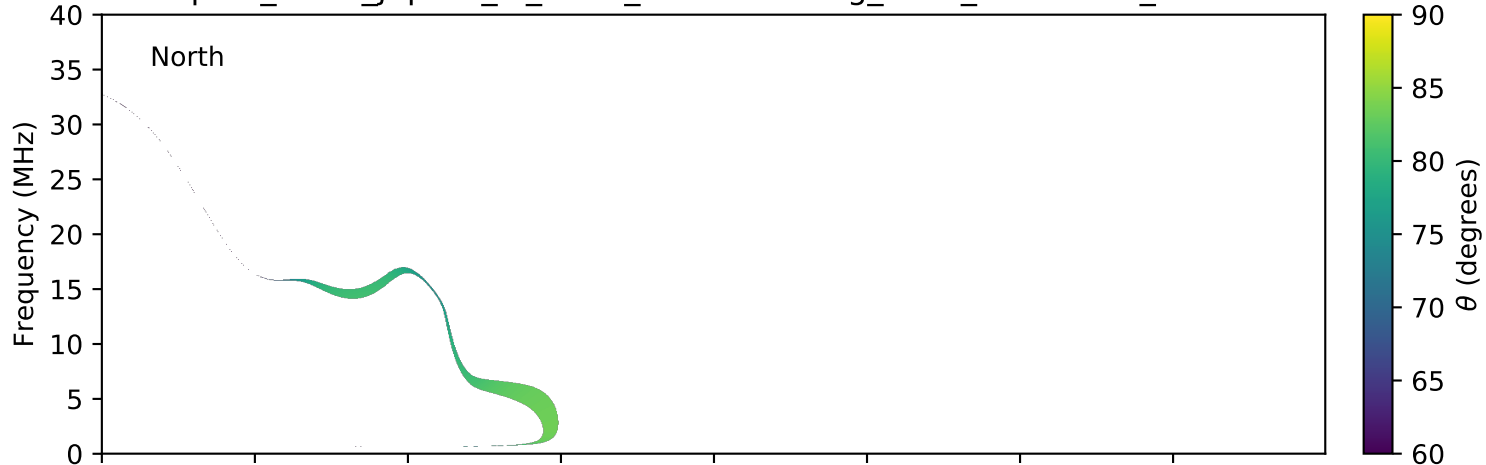
expres_earth_jupiter_io_isaac_lossc-wid1deg_3kev_20160416_v01.cdf
