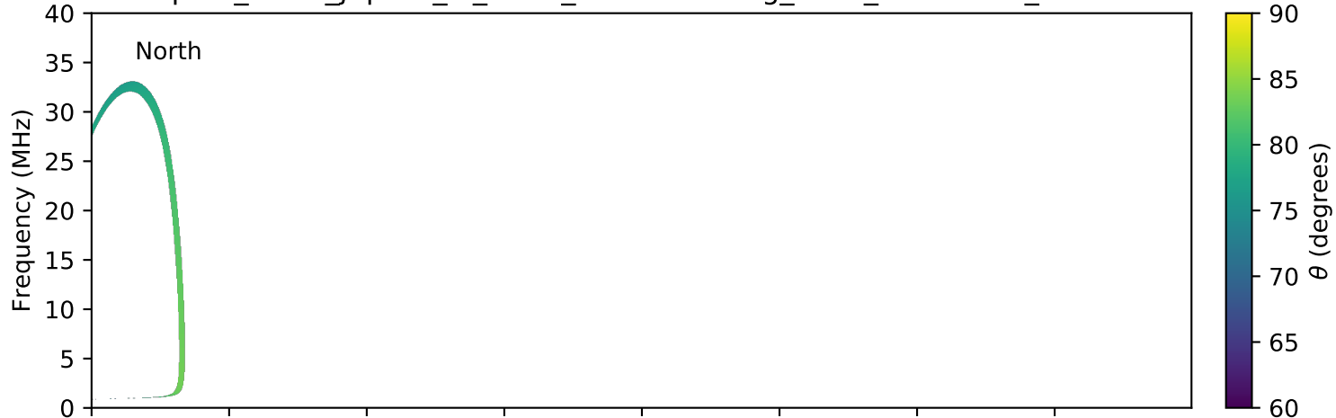
expres_earth_jupiter_io_isaac_lossc-wid1deg_3kev_20160411_v01.cdf
