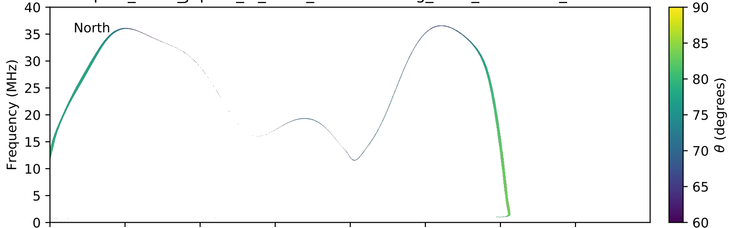
expres_earth_jupiter_io_isaac_lossc-wid1deg_3kev_20160405_v01.cdf
