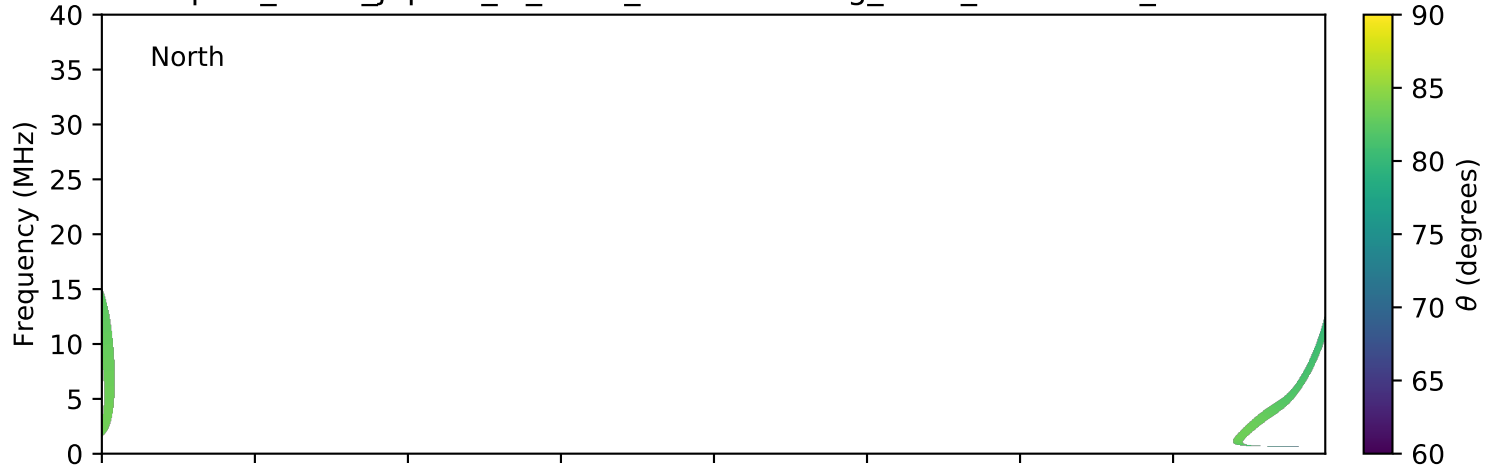
expres_earth_jupiter_io_isaac_lossc-wid1deg_3kev_20160404_v01.cdf
