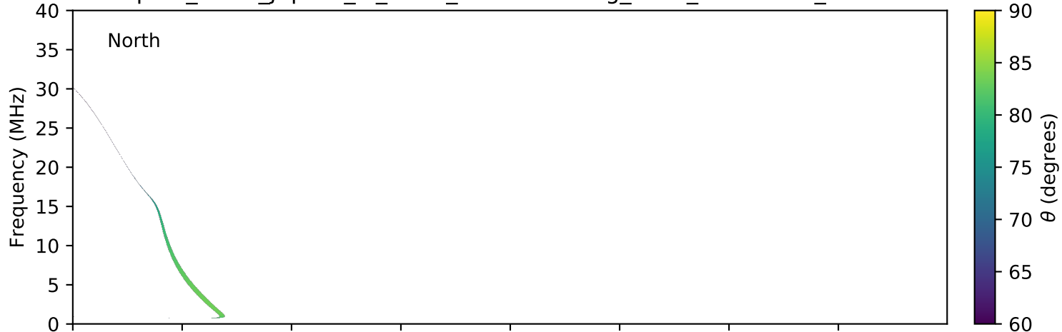
expres_earth_jupiter_io_isaac_lossc-wid1deg_3kev_20160402_v01.cdf
