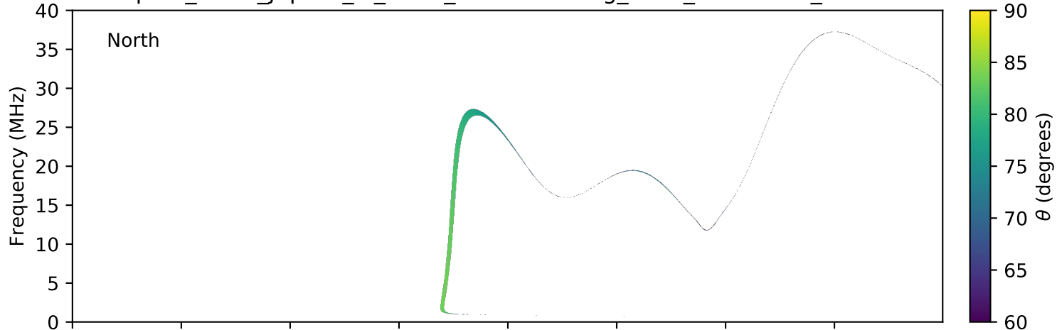
expres_earth_jupiter_io_isaac_lossc-wid1deg_3kev_20160401_v01.cdf
