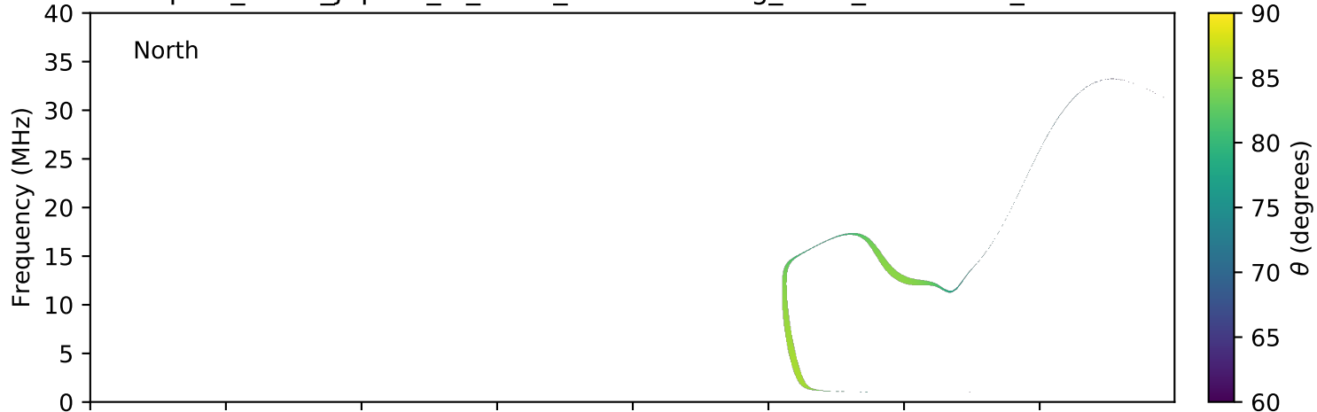
expres_earth_jupiter_io_isaac_lossc-wid1deg_1kev_20160429_v01.cdf
