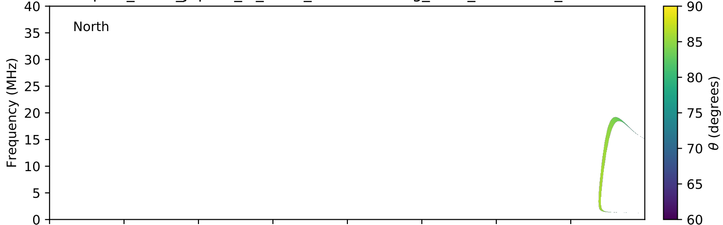
expres_earth_jupiter_io_isaac_lossc-wid1deg_1kev_20160427_v01.cdf
