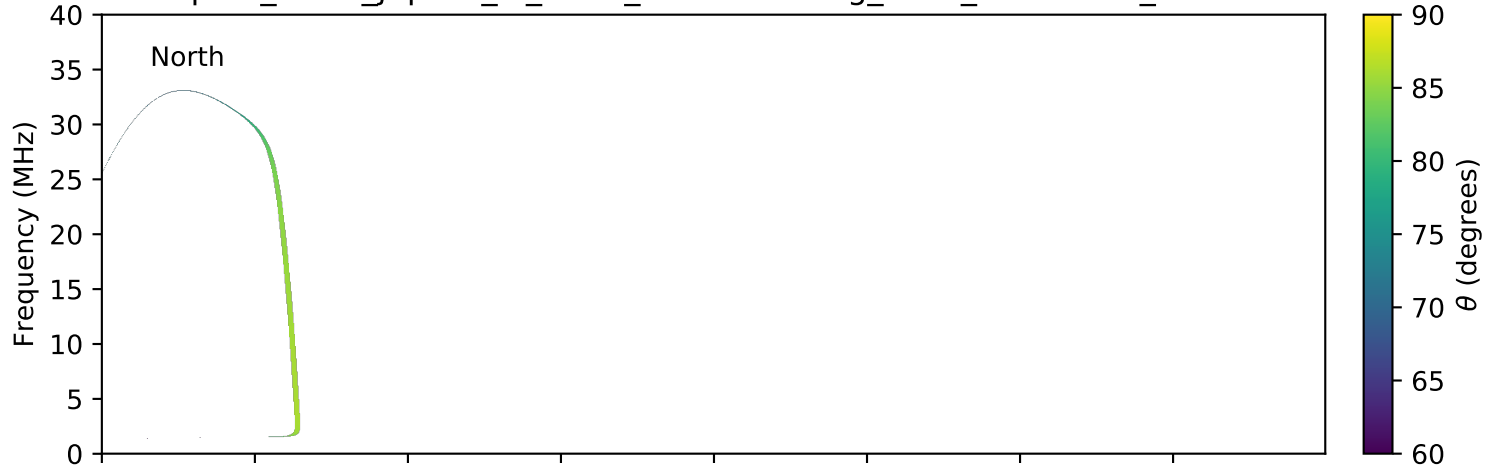
expres_earth_jupiter_io_isaac_lossc-wid1deg_1kev_20160418_v01.cdf
