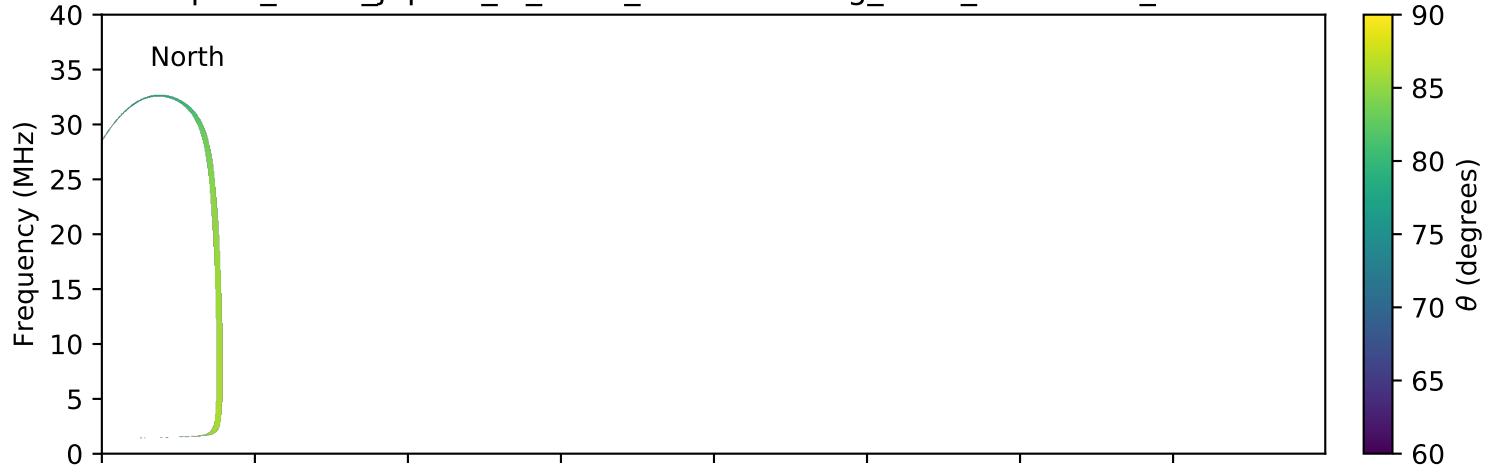
expres_earth_jupiter_io_isaac_lossc-wid1deg_1kev_20160411_v01.cdf
