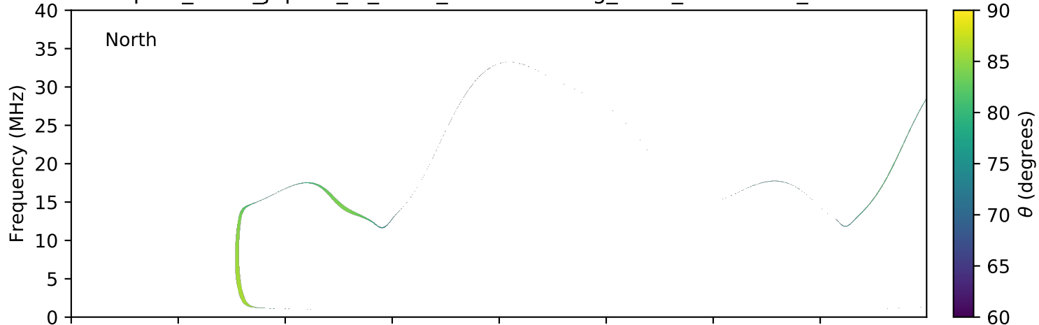
expres_earth_jupiter_io_isaac_lossc-wid1deg_1kev_20160410_v01.cdf
