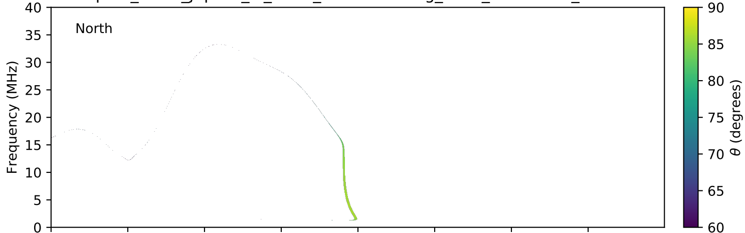
expres_earth_jupiter_io_isaac_lossc-wid1deg_1kev_20160407_v01.cdf
