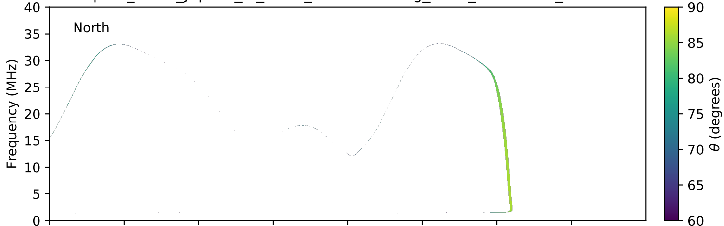
expres_earth_jupiter_io_isaac_lossc-wid1deg_1kev_20160405_v01.cdf
