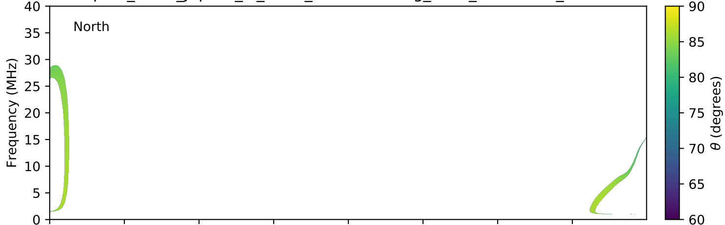
expres_earth_jupiter_io_isaac_lossc-wid1deg_1kev_20160404_v01.cdf
