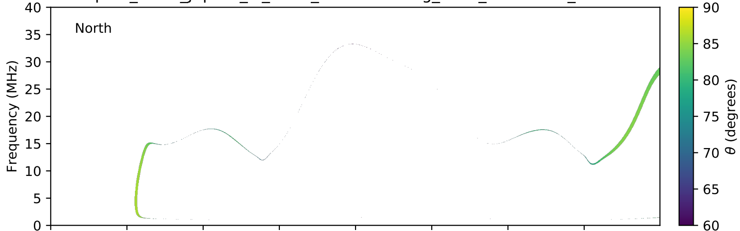
expres_earth_jupiter_io_isaac_lossc-wid1deg_1kev_20160403_v01.cdf
