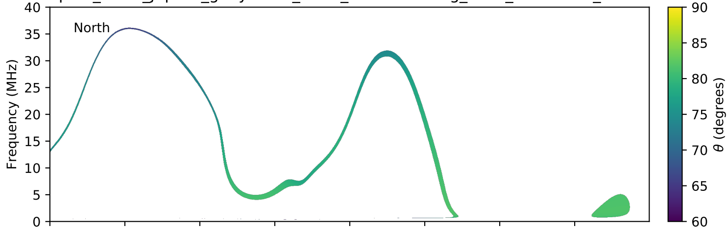
expres_earth_jupiter_ganymede_isaac_lossc-wid1deg_5kev_20160408_v01.cdf
