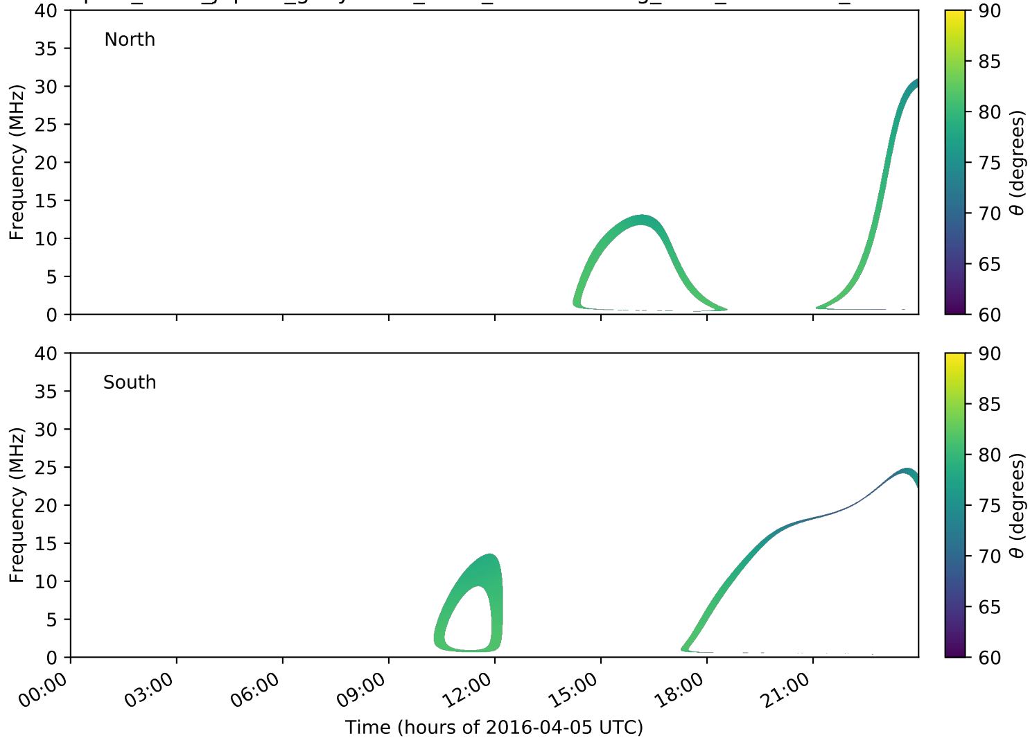
expres_earth_jupiter_ganymede_isaac_lossc-wid1deg_5kev_20160405_v01.cdf
