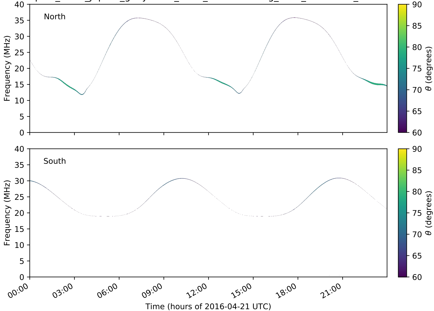
expres_earth_jupiter_ganymede_isaac_lossc-wid1deg_3kev_20160421_v01.cdf
