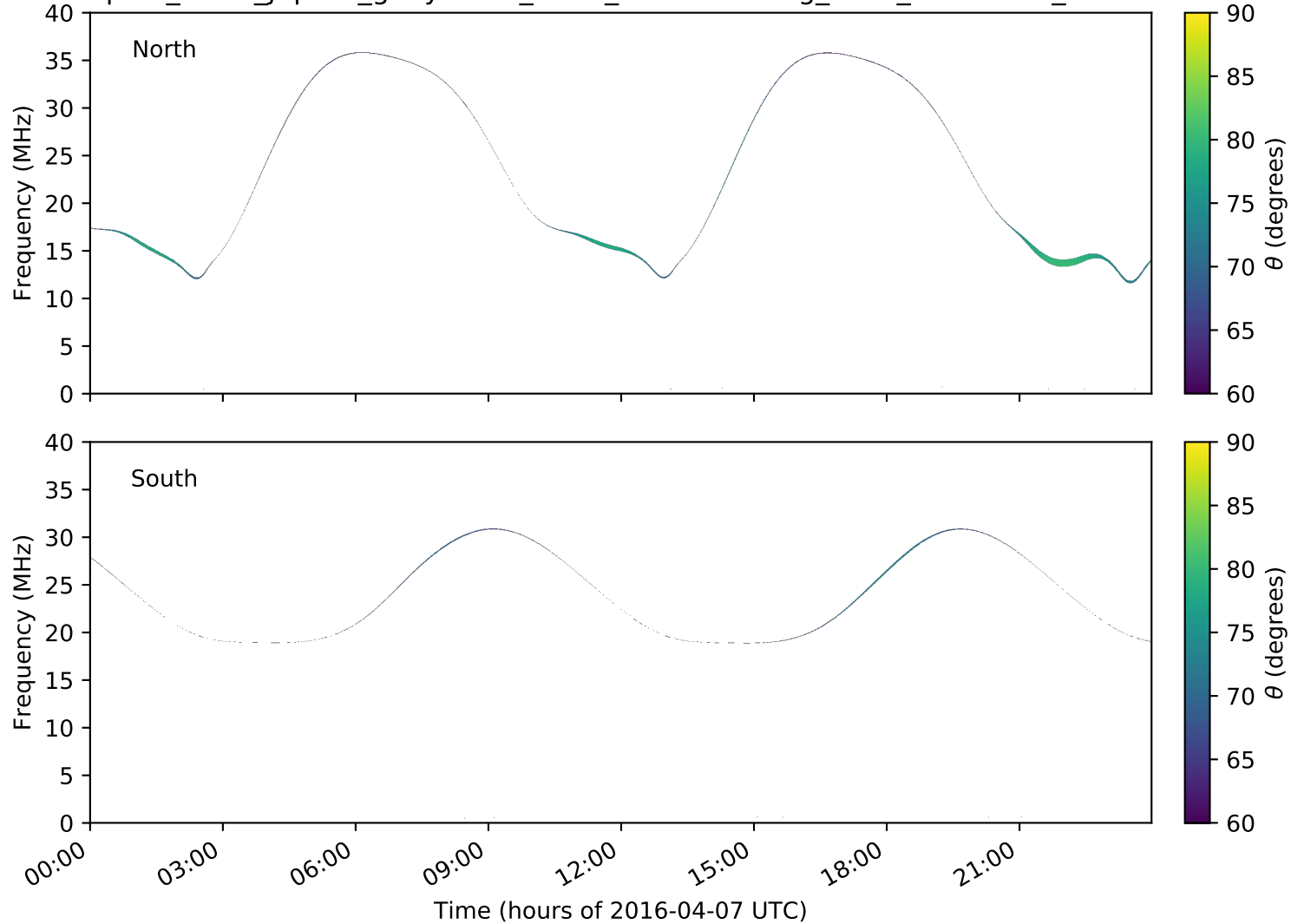
expres_earth_jupiter_ganymede_isaac_lossc-wid1deg_3kev_20160407_v01.cdf
