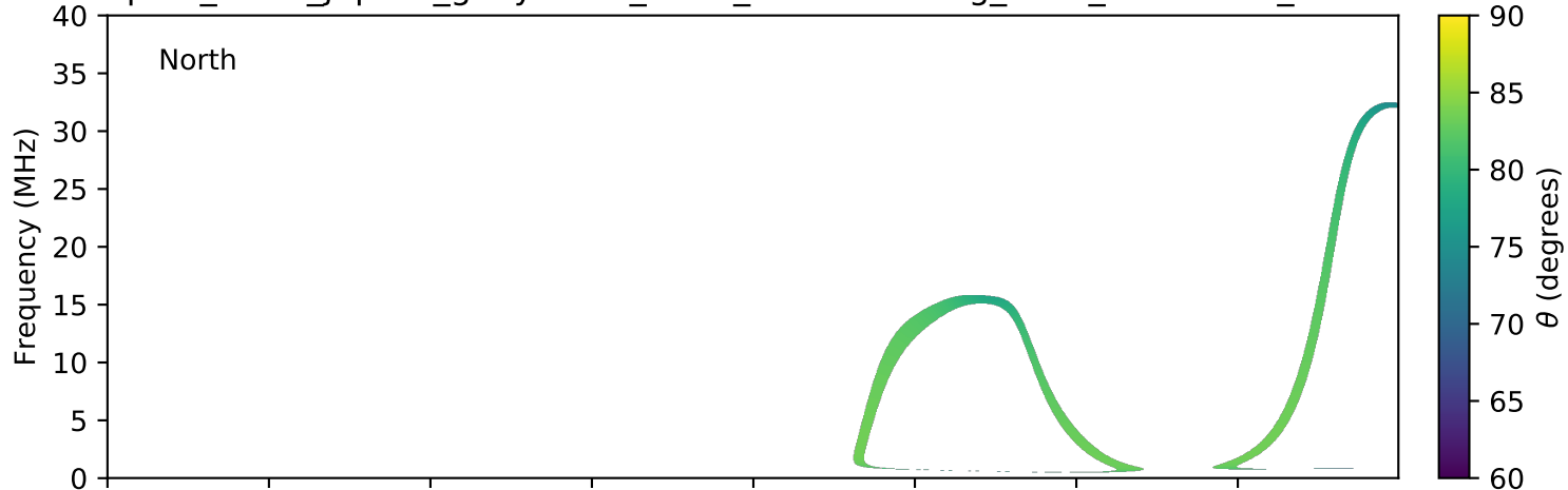
expres_earth_jupiter_ganymede_isaac_lossc-wid1deg_3kev_20160405_v01.cdf
