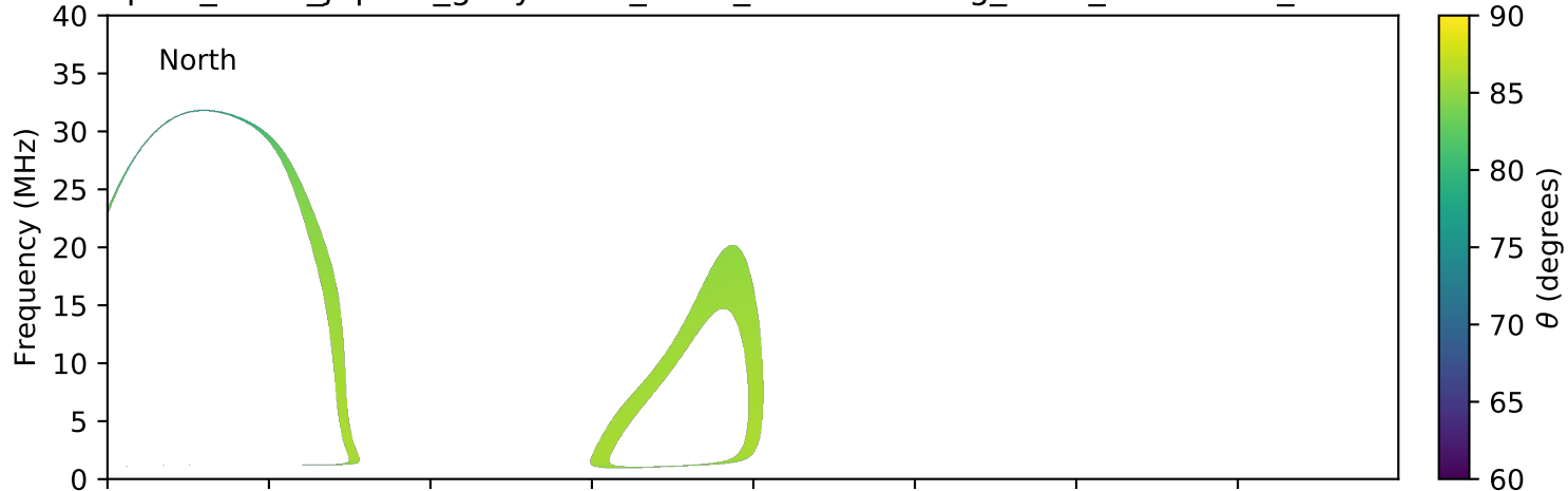
expres_earth_jupiter_ganymede_isaac_lossc-wid1deg_1kev_20160430_v01.cdf
