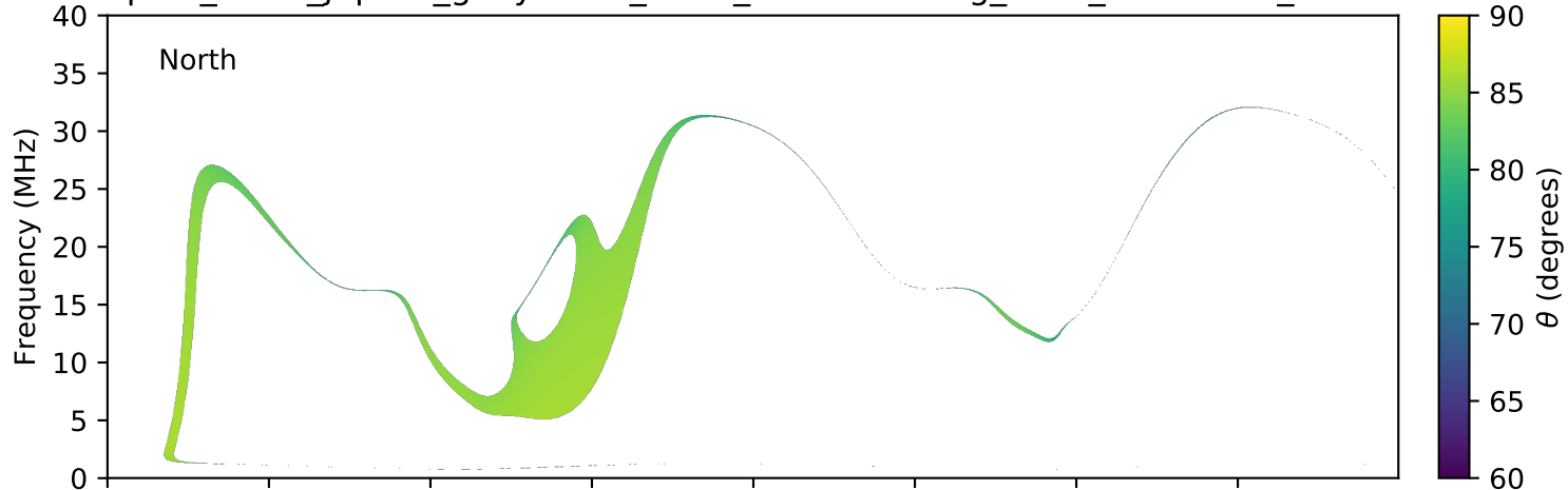
expres_earth_jupiter_ganymede_isaac_lossc-wid1deg_1kev_20160427_v01.cdf
