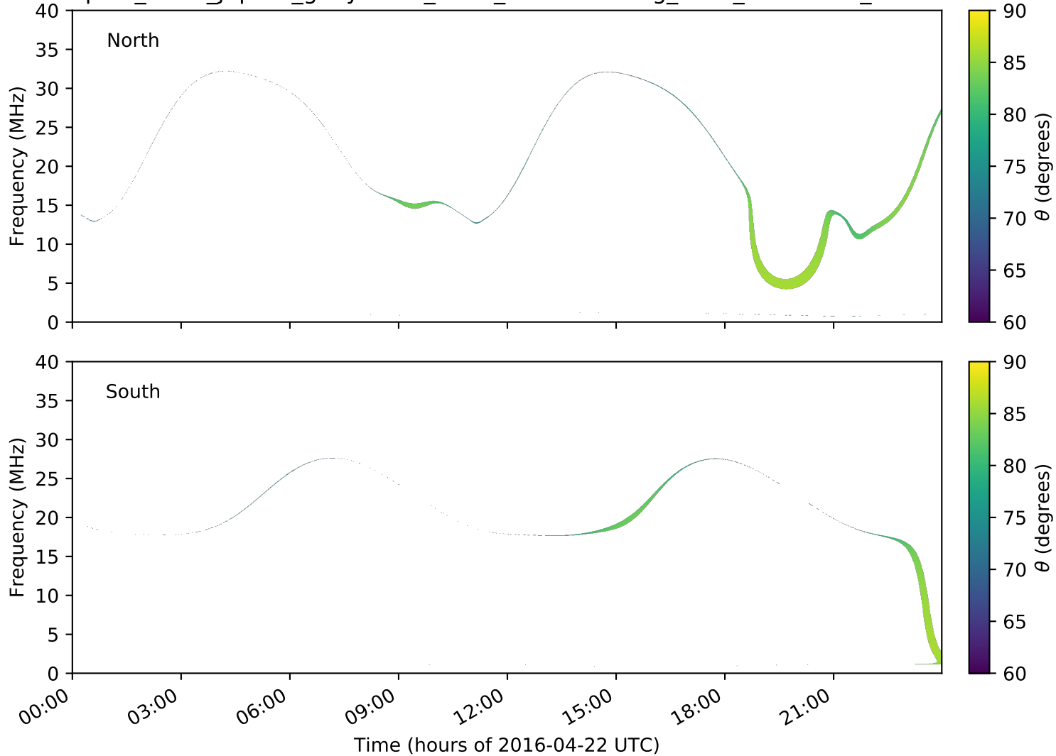
expres_earth_jupiter_ganymede_isaac_lossc-wid1deg_1kev_20160422_v01.cdf
